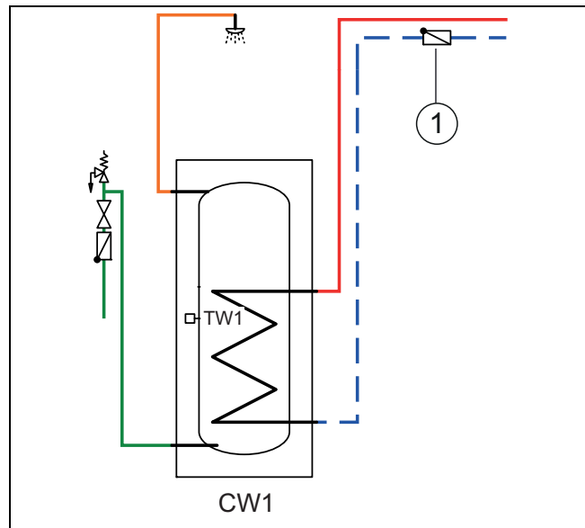
Afb. 21 Boiler
