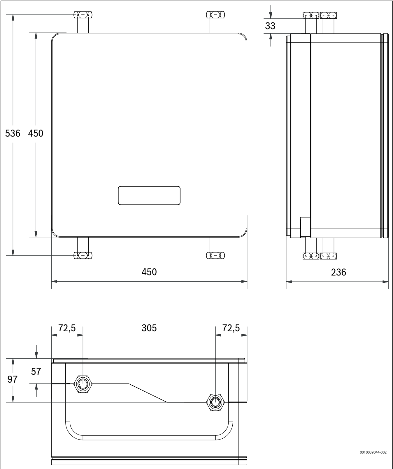
Fig. 3 Dimensions, raccordements
